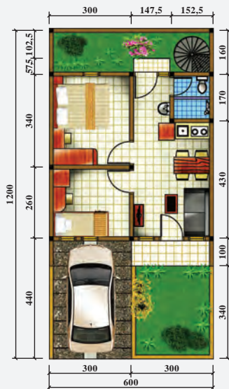
Denah Lantai 1
