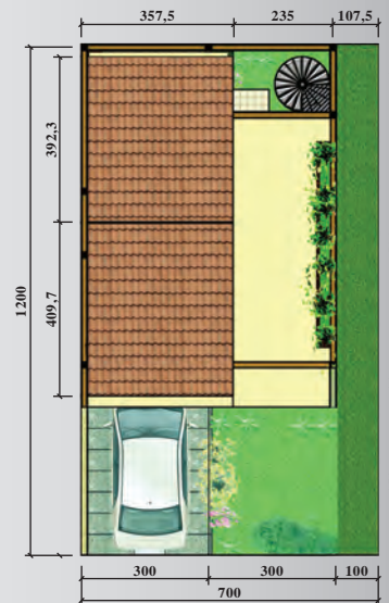
Denah Lantai 2
