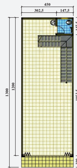
Denah Lantai 1
