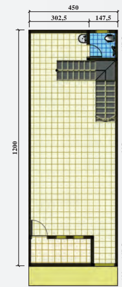
Denah Lantai 2
